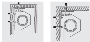
Installation bracket for screens 150' and above
