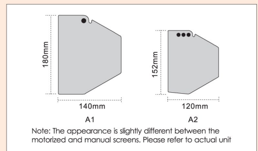
Installation bracket for screens under 150'
